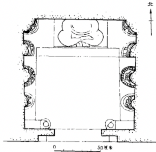
Illustration 1: Sketch of Xiaonanhai middle cave's structure, from: Henan Sheng gudai jianzhu baohu yanjiusuo 河南省古代建築保護研究所, “Henan Anyang Lingquansi shiku ji Xiaonanhai shiku 河南安陽靈泉寺石窟及小南海石窟,” Wenwu 文物 (1988/4), page 11 (figure 36).
