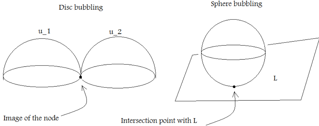
Figure 1.1: The codimension one boundary in \overline{\mathcal{M}}_{k,l}^{\text{disc}}(X, L, \beta)
