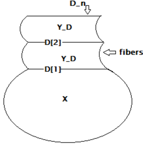
Figure 4.1: The singular manifold X[n] .
