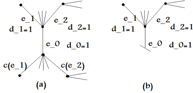
Figure 6.1: A typical decorated graph (a) and its half (b).
