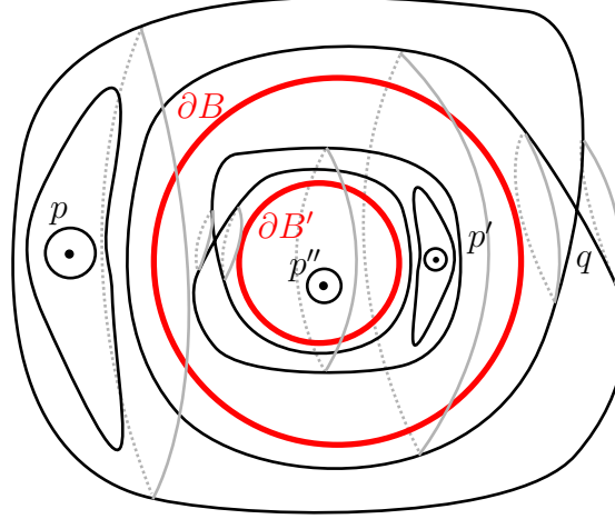
Figure 4.2: Starting from dot p and flowing perpendicular to the singular fibration \mathcal{F} , the next singular leaf we find has a cone q corresponding to an index-2 critical point. A nearby leaf component is a sphere bounding ball B containing dot p' . Starting from p' and flowing perpendicular to the leaves of \mathcal{F} , again the first cone corresponds to a critical point of index-2. A nearby leaf component is a sphere bounding ball B' \subset B containing dot p'' .
