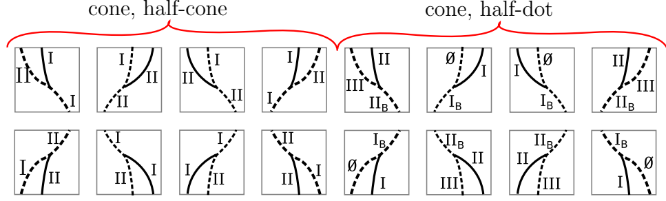
Figure 3.18: Top row: valid singularity charts for the cone, half-cone and cone, half-dot deaths. Bottom row: valid singularity charts for the cone, half-cone and cone, half-dot births. We omit the arc of the half-cone or half-dot which is not cancelled or born during the movie.
