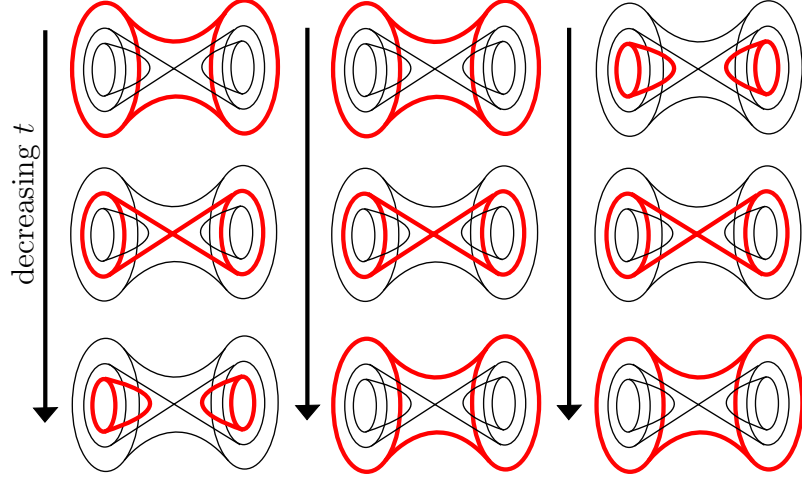
Figure 2.3: Left and right: cross-sections of a smooth 3-manifold. Each has one singular cross-section (containing a cone). The nearby cross-sections are different resolutions of that cone. Middle: cross-sections of a singular 3-manifold. Even though there is only an isolated singular cross-section (a single cone), the resolutions of the cone are the same above and below the singular cross-section.
