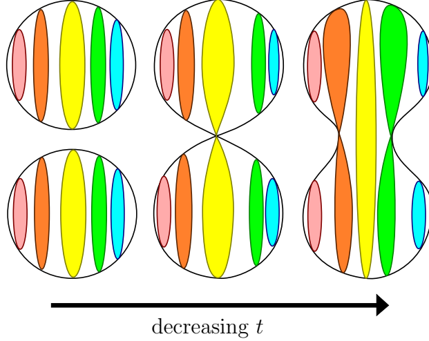
Figure 3.8: The third boundary fusion movie.
