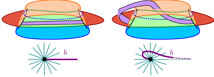
Figure 1.3: Top left: a band b lies in a single Seifert surface for a fibered knot K . Top right: Perturb the band near one component of b \cap K so that \mathring{b} is transverse to each leaf. (We can think of this perturbation as going halfway around S^1 = \pi(S^3 \setminus K) , where \pi is the projection map from S^3 = \mathring{\Sigma} \times_{\phi} S^1 to S^1 .) Bottom left: side view of b in one leaf, near one end of b \cap K . Bottom right: side view after perturbing b .
