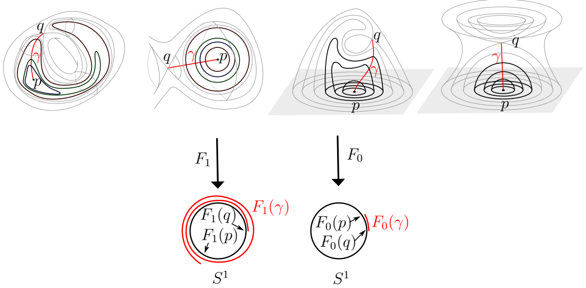
Figure 3.13: Diagram of positioning a dot or half-dot. We draw a neighborhood of B , which might be a solid torus or a ball. On the light gray leaf components (and all components not illustrated), \mathcal{F}_t is fixed for all t . As t decreases, the range of \mathcal{F}_t(B) contracts.
