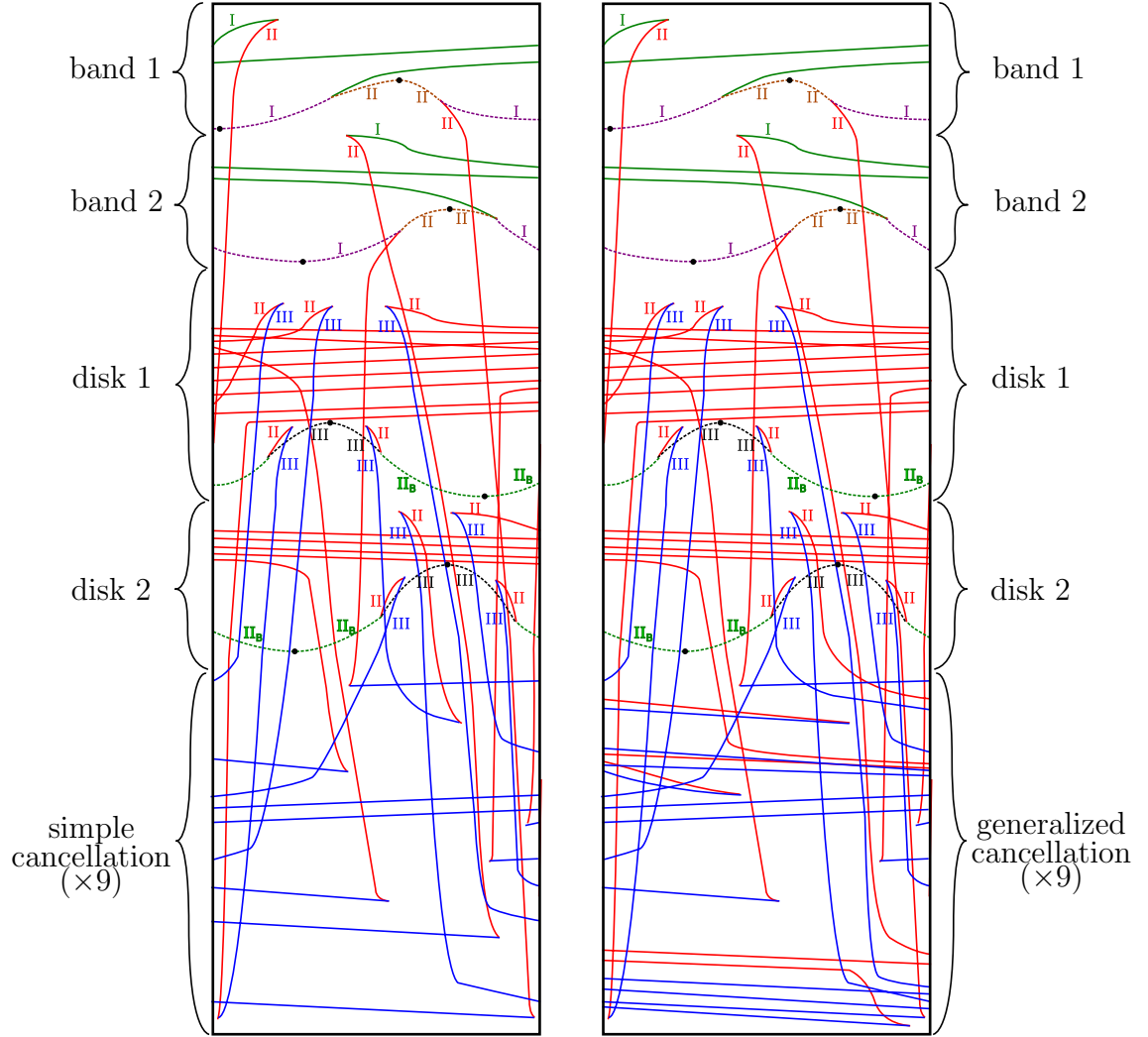
Figure 3.31: A possible valid singularity chart for \mathcal{F}_t when \mathcal{F}_t is a composition of two band movies, two disk movie, and then nine cancellation movies. Left: All cancellations are simple. Right: The cancellations are generalized.
