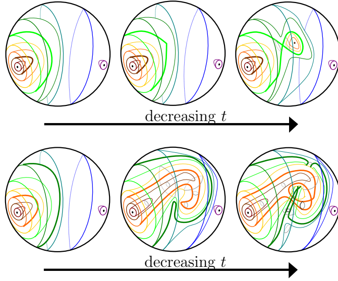
Figure 3.1: A diagram of an interior stabilization movie. As t decreases, we perturb \mathcal{F}_t to add a cancelling pair of critical points. Top: an index-0,-1 or -2,-3 pair, depending on the orientation of \mathcal{F}_t . Bottom: an index-1,-2 pair (the order depends on the orientation of \mathcal{F}_t ).
