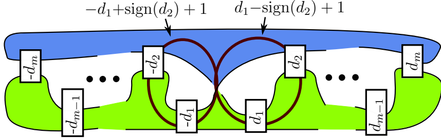
Figure 6.4: A minimum-genus Seifert surface for 2-bridge ribbon knots in Family 1. From this surface, we can deplumb annuli with d_1 - \text{sign}(d_2) + 1 and -d_1 + \text{sign}(d_2) + 1 half-twists. These cannot both be Hopf bands, so the surface is not a fiber (and hence the knot is not a fibered knot).
