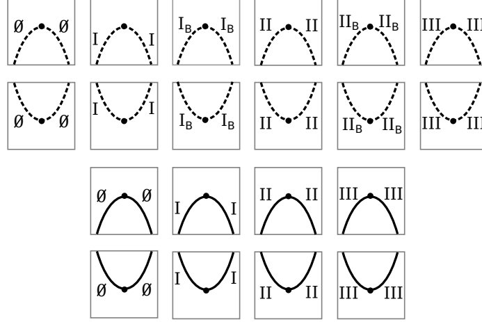
Figure 3.12: Valid singularity charts for the boundary fusion, compression, birth, death and interior singularity movies.
