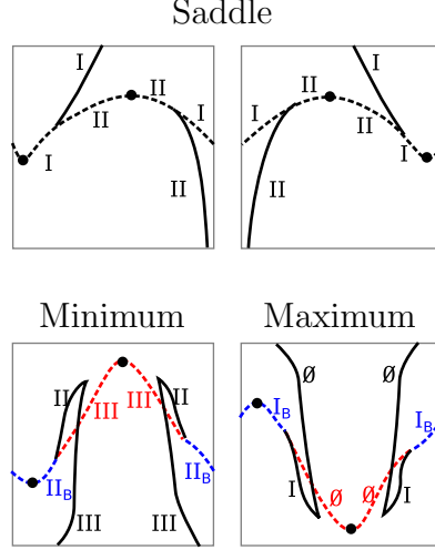
Figure 3.21: Top row: two singularity charts for the saddle movies (the difference is the indices of the singular points). Bottom left: a chart for the minimum movie. Bottom right: a chart for the maximum movie. The colors are just meant to help the reader distinguish intersecting arcs. We omit arcs corresponding to singularities which persist from t = 1 to t = 0 .
