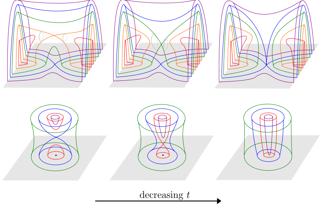
Figure 3.17: Top: a schematic of the cone, half-cone death. Bottom: a cone, half-dot death.
