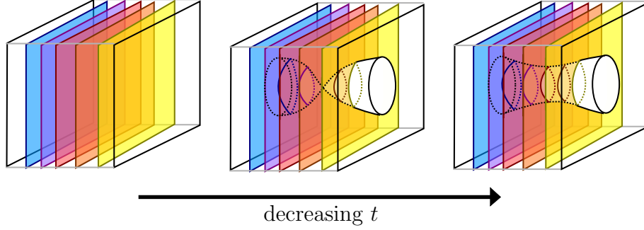
Figure 3.7: The second boundary fusion movie. We only draw a neighborhood of the arc between the two bowls, ignoring the other boundary singularities.
