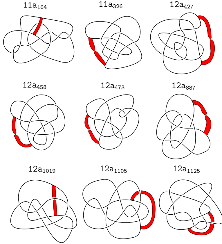
Figure 6.2: A band diagram of a 2-minimum disk for each knot of Fig. 6.1 except 12a_{990} , constructed by B. Owens and F. Swenton.
