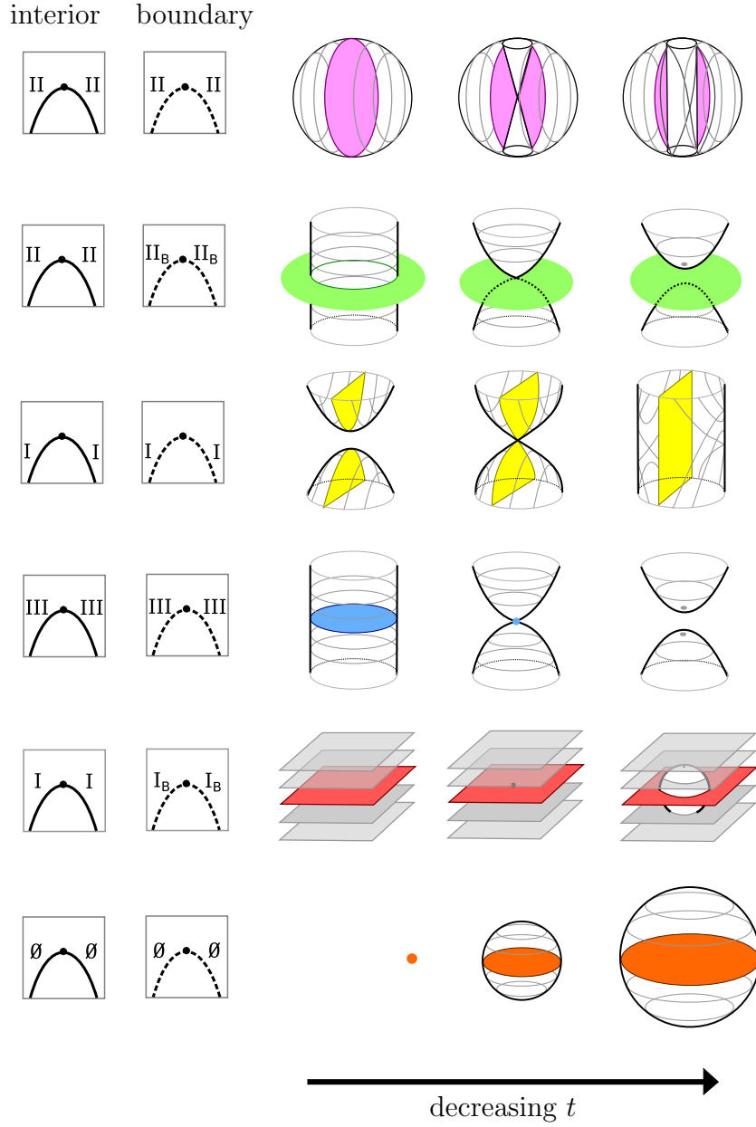
Figure 2.7: If \mathcal{F}_t has a valid movie of singular fibrations, then near a critical point of h , \mathcal{F}_t looks like one of these movies or their inverses ( t \mapsto 1 - t ). We shade the H_\theta that includes the critical point of h , and find that H_\theta is smooth near the critical point. We have drawn each picture as if the singularity is in \partial M^3 ; double the picture to obtain a movie containing an interior critical point of h .
