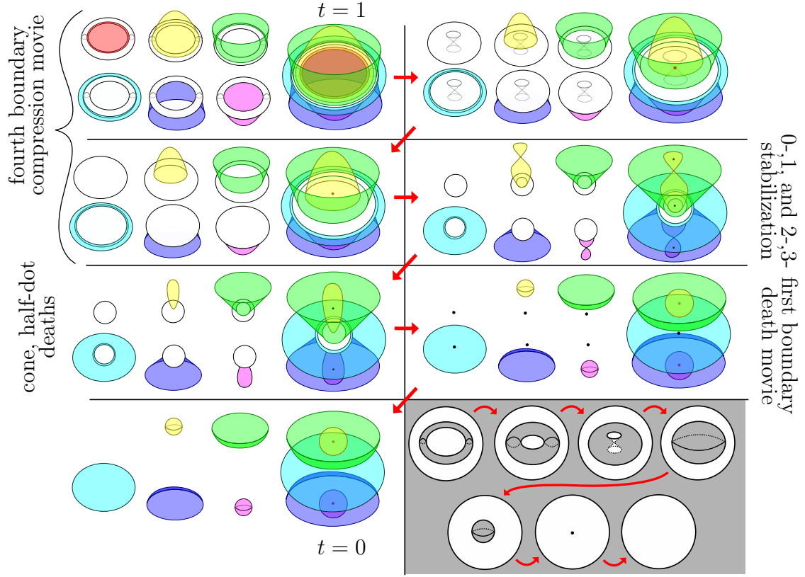
Figure 3.20: Diagram of a minimum movie. This is a movie of singular fibrations on (B^3 \times I) \setminus \nu(\text{disk with one minimum}) .
