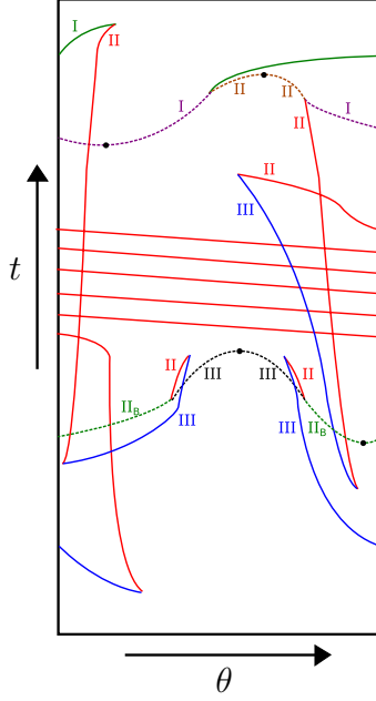
Figure 2.6: An example of a valid singularity chart. Note that no arc is ever vertical. Each endpoint locally looks like one of the images in Fig. 2.5. Colors/shades of the arcs are only meant to help the reader view the image; they contain no mathematical meaning.
