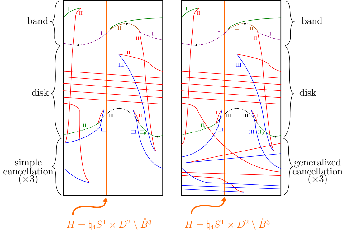
Figure 5.1: We draw potential valid singularity charts for \mathcal{F}_t , t \in [s_{n+1}, 3] . By Lemma 4.2, we may assume that the cancellations of \mathcal{F}_t are all simple, as on the left. Then all 2-handles of H arise from positioning a cone or playing a minimum movie during a disk movie. Therefore, the 2-handles are attached exactly along the intersections of \mathcal{F}_t^{-1}(\theta) with a minimum disk, projected to the same height.
