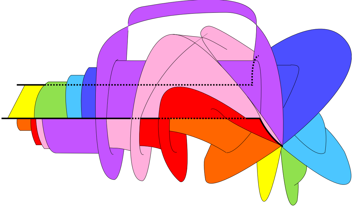
Figure 3.26: A detailed view of a cone singularity in \mathcal{G}_0 near the end of band b in a band movie. The two cones have identical neighborhoods, modulo rotation.
