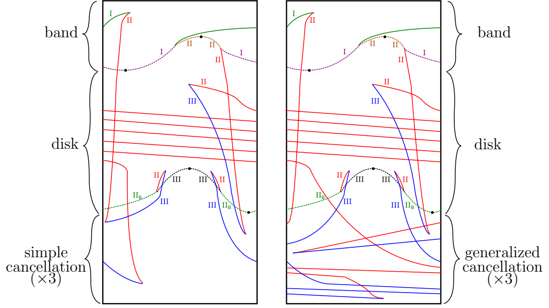
Figure 3.30: A possible valid singularity chart for \mathcal{F}_t when \mathcal{F}_t is a composition of one band movie, one disk movie, and then three cancellation movies. Left: All cancellations are simple. Right: The cancellations are generalized.
