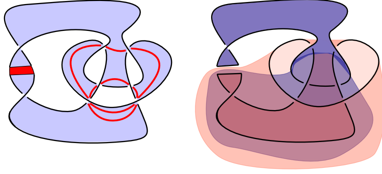
Figure 5.2: Left: The fibered knot K = 8_{20} (i.e. the pretzel knot P(2, -3, 3) ). We draw a fission band defining a ribbon disk D with boundary K and shade a genus-2 fiber surface for K . On the fiber, we draw two attaching circles defining a genus-2 handlebody fiber of B^4 \setminus \nu(D) . Right: Two disjoint disks bounded by K resolved along the fission band. These disks intersect the fiber in arcs (near the band) and two curves, which are the attaching circles drawn on the left.
