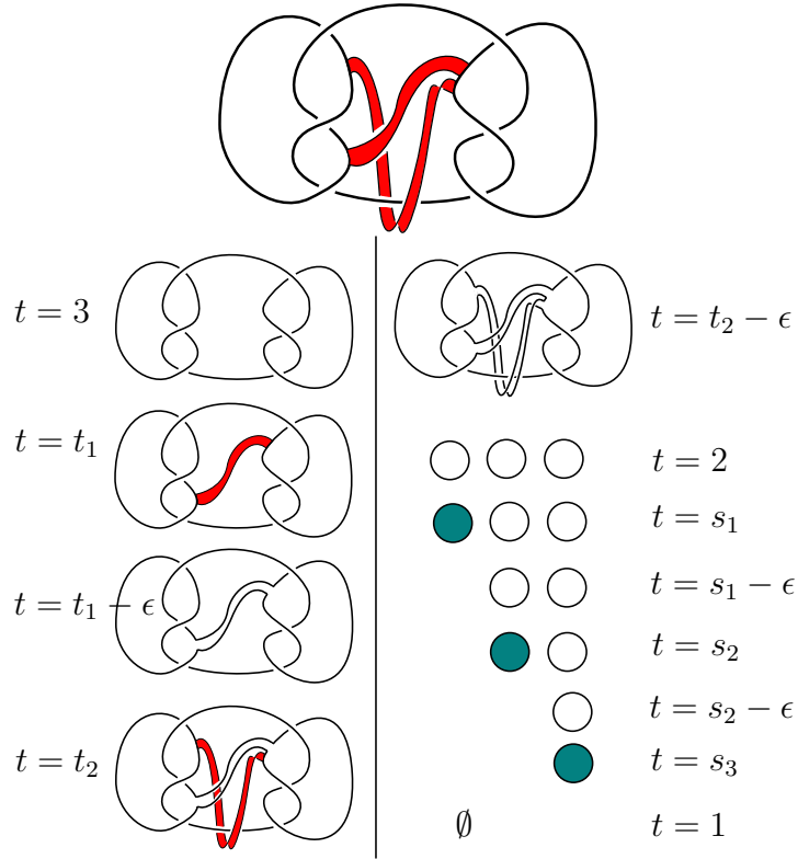
Figure 1.1: Top: a diagram of a ribbon disk D with boundary the square knot. Below: Some cross-sections of D \subset B^4 . Recall h^{-1}(3) (that is, t = 3 ) is the boundary S^3 of B^4 .
