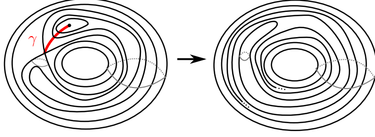
Figure 3.22: If we attempt to cancel a dot with a cone where the two sheets of \mathcal{F}_t^{-1}(\theta) near the cone are in the same component of \mathcal{F}_t^{-1}(\theta) , then we cannot actually destabilize the circular Morse function \mathcal{F}_t . Left: a local picture of a dot and cone singularity; the two sheets of a leaf near the cone are in the same component of the leaf. Right: We attempt to cancel the dot and cone singularities and create a Reeb component, which is not allowed in the definition of a singular fibration.
