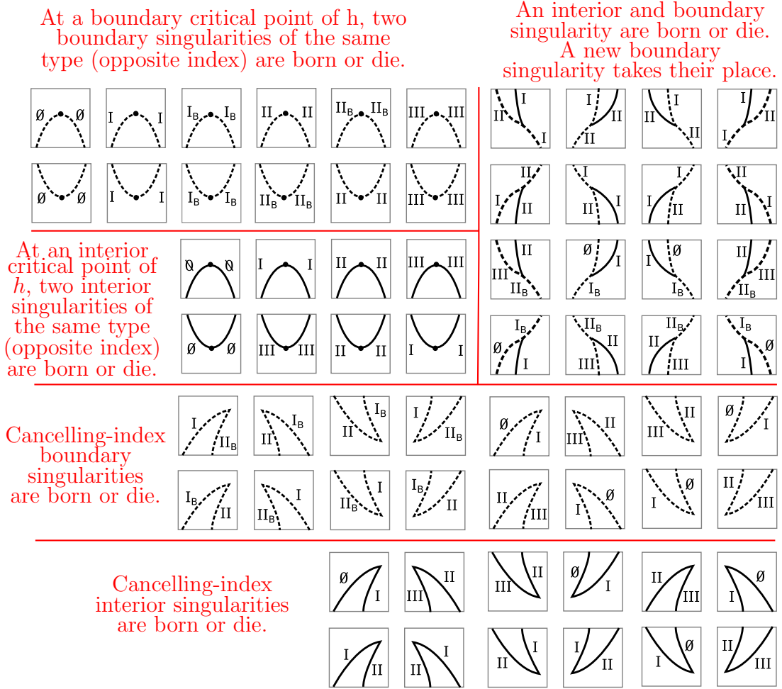
Figure 2.5: Possible configurations of two or three arcs meeting at an endpoint in a valid singularity chart.
