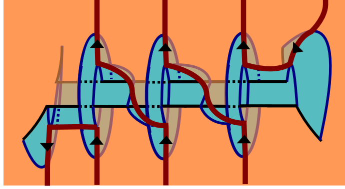
Figure 4.3: Rectangular sheet: part of the minimum disk d_i which intersects a core of the band b_j . Surface: A leaf L of \mathcal{F}_t for t = t_i - \epsilon . Some curves in L \cap d_i run along the cores of the 1-handles corresponding to b_j (attached to the 3-dimensional fiber H ). These curves are all distinct, since they locally have the same orientation in d_i (Here, we are using the fact that b_j is transverse to the fibration \mathcal{F}_t ). Therefore, 2-handles attached to H corresponding to the Type II cones arising during the disk movie on d_i will geometrically cancel the 1-handles corresponding to the type I cones arising during the band movie on b_j .
