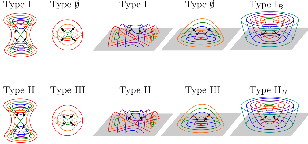
Figure 2.4: The type of a singularity p of \mathcal{F}_t . The arrow indicates the direction in which a singular cross-section of H_\theta is resolved as t decreases.
