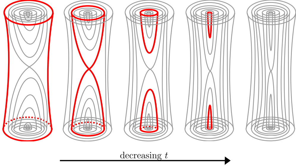
Figure 3.15: When positioning a cone along an arc \gamma , suppose \gamma meets no other singular leaf. By reparametrizing \mathcal{F}_t , we find a movie \mathcal{G}_t in which the positioned cone is type II. In bold: \mathcal{G}_t^{-1}(\theta_0) near the positioned cone, as t decreases.
