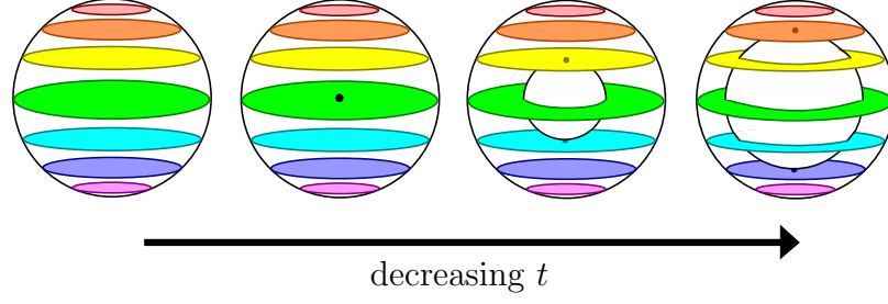
Figure 3.10: The first boundary birth movie.
