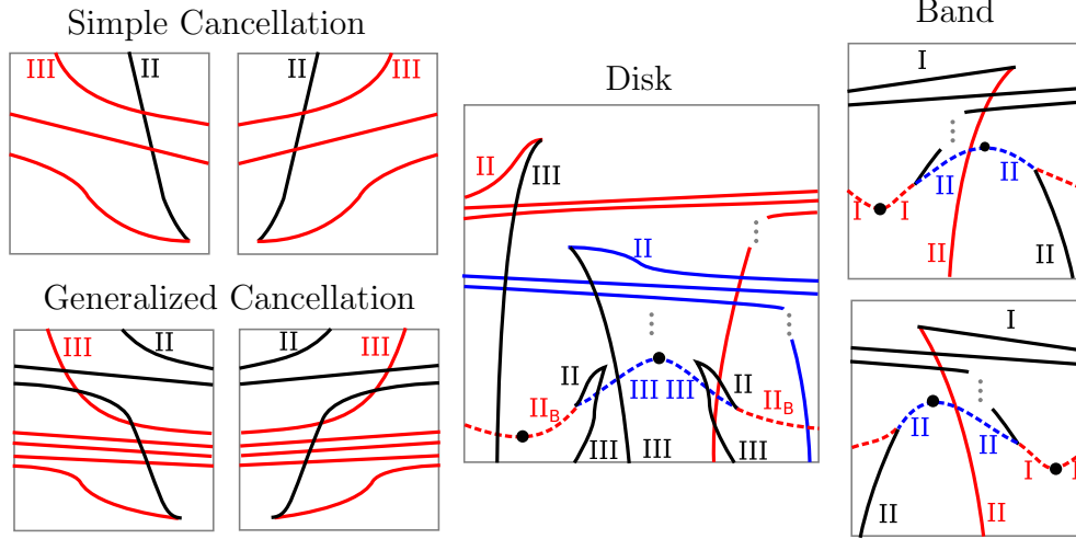
Figure 3.29: Top left: two singularity charts for the simplified cancellation movie, depending on the indices of the cancelled singularities. Bottom left: two singularity charts for the generalized cancellation movie. Middle: A potential chart for the disk movie, where we included one 0,1- stabilization and one 2,3-stabilization (recall these choices depend on orientations of leaves of \mathcal{F}_1 intersecting the disk). Right: two singularity charts for the band movie (recall the types of the cones created in the 1-2- stabilization depends on the orientation of \mathcal{F} ).
