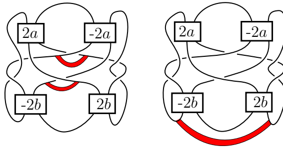
Figure 6.3: Left: bands defining a ribbon disk for K \subset S^3 , constructed by Lisca [19]. Right: A 2-minimum ribbon disk with the same boundary knot. Note here that the integers \pm 2a, \pm 2b refer to half-twists. The knot K is fibered if and only if |a| = |b| = 1 .
