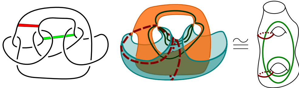
Figure 5.3: Left: A diagram for the fibered ribbon knot K = 11n_{74} (i.e. the pretzel knot P(3, -3, 3, -2) ). Each of the pictured bands specifies a 2-minimum ribbon disk D_i for K . (These examples of disks come from [20], who produce many examples of doubly slice knots.) Using the construction of Theorem 1.8, we find attaching circles for the handlebody fiber for each disk. Middle: The fiber F for K consists of two annuli glued along three half-twisted bands. The two sets of circles specify the handlebody fiber for the disks given by the bands. Right: On F \cup D , the attaching circles specify a Heegaard splitting of S^3 . Thus, D_1 \cup \overline{D_2} \subset S^4 is fibered by 3-balls (so D_1 \cup \overline{D_2} is the unknotted sphere).
