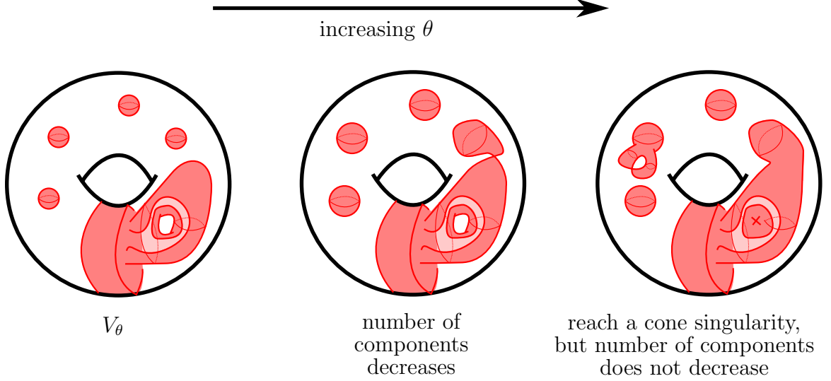
Figure 4.1: Schematic of V_\theta for increasing \theta . Left: V_\theta for \theta > 0 small. Middle: The number of components of V_\theta decreases. \mathcal{F}^{-1}(\theta) contains a cone satisfying the second condition of the proposition. Right: We draw two cones. One is index-2, one is index-1 but does not satisfy the other condition. The number of components of V_\theta does not decrease.
