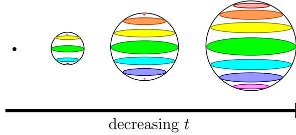
Figure 3.11: The second boundary birth movie.
