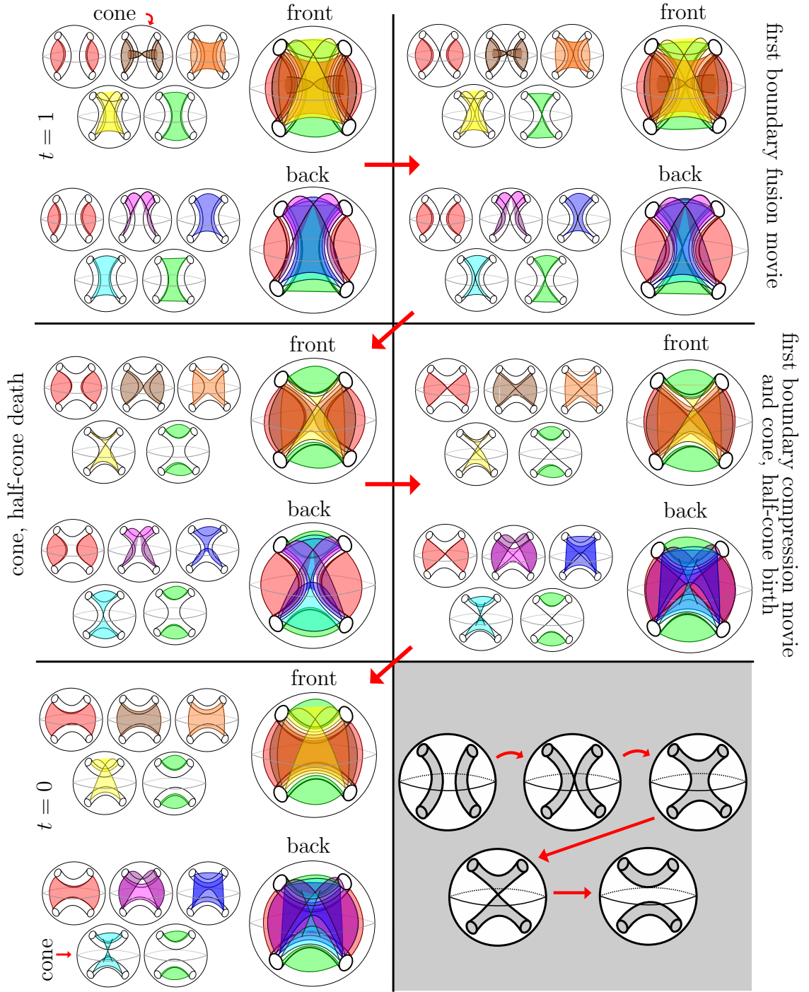
Figure 3.19: Diagram of a saddle movie. This is a movie of singular fibrations on (B^3 \times I) \setminus \nu(\text{saddle}) .
