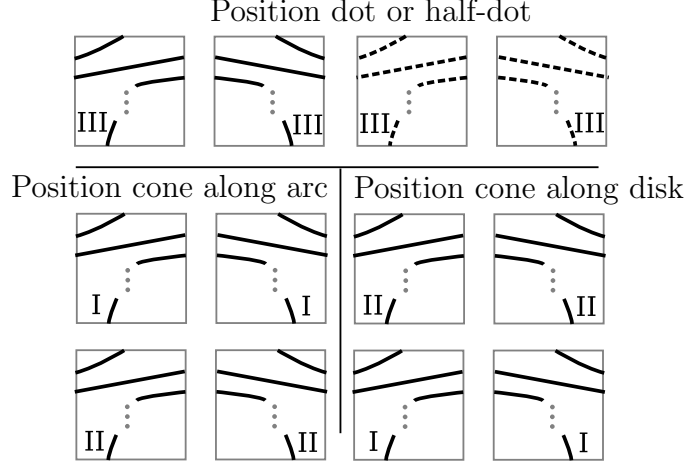
Figure 3.16: Valid singularity charts for the positioning movies. Each chart contains one arc (we omit the arcs of the singularities we are not positioning).
