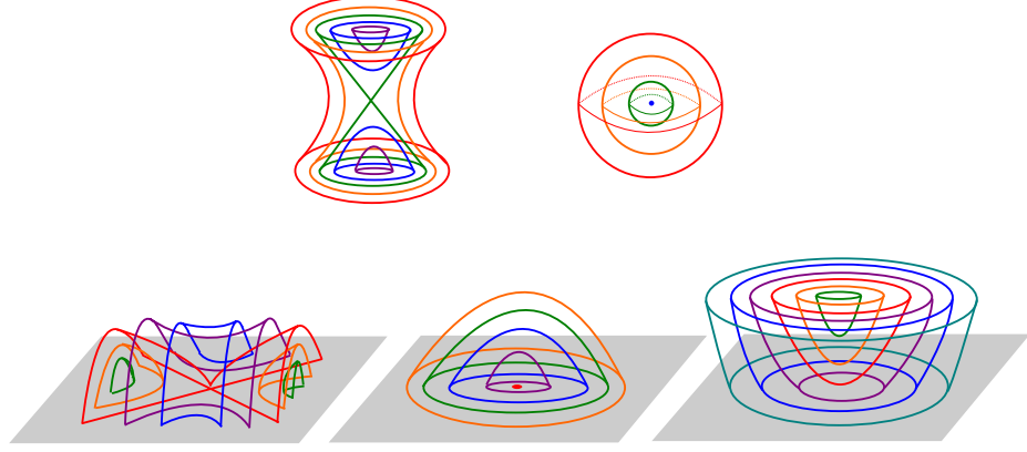
Figure 2.1: Top: neighborhoods of a cone and dot singularity in \mathring{M}^3 . Bottom: Leaves of \mathcal{F} near a half-cone, half-dot, and bowl singular point in the foliation induced on \partial M^3 .
