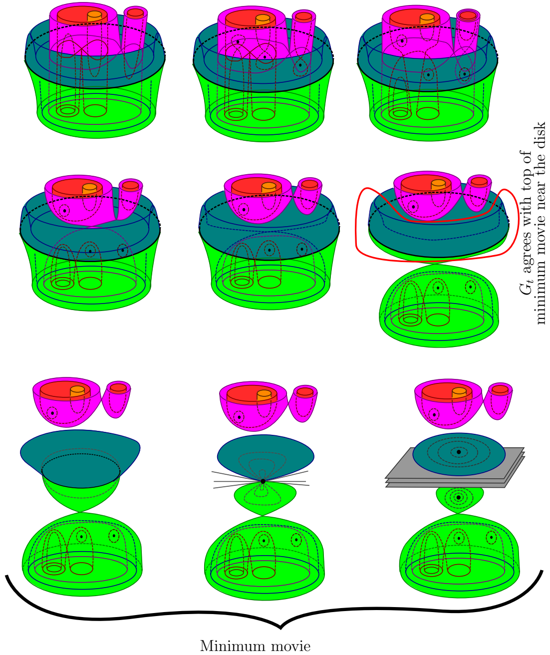
Figure 3.27: Left to right, top to bottom: Some leaves of \mathcal{G}_t as t decreases from 1 to 0 in a disk movie. As t decreases, we perform interior stabilizations and position the cones along disks until in a set B containing \partial D in h^{-1}(1/4) , \mathcal{G}_{1/4} agrees with the top of the minimum movie. We play the minimum movie from t = 1/4 to 0.
