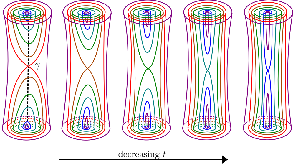
Figure 3.14: Diagram of positioning a cone along an arc \gamma . We draw a neighborhood of \gamma . As t decreases, the value of \mathcal{F}_t(\text{cone point}) changes from \mathcal{F}_1(\gamma(0)) to \mathcal{F}_1(\gamma(\pm 1)) .
