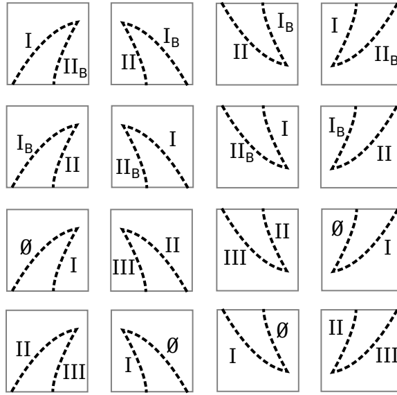
Figure 3.5: Valid singularity charts for each boundary stabilization/destabilization. The left half are boundary stabilization, while the right half are boundary destabilization. Top and second row: 1-, 2- (de)stabilization. Third row: 0-, 1-(de)stabilization. Bottom row: 2-, 3-(de)stabilization.
