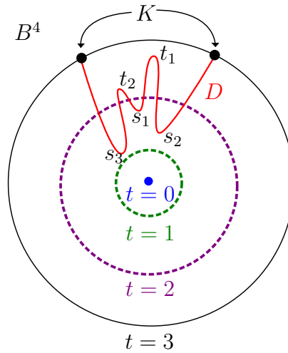
Figure 1.2: A schematic of a ribbon disk in B^4 . In this example, the disk has 3 minima and 2 index-1 critical points (bands), as in Figure 1.1.
