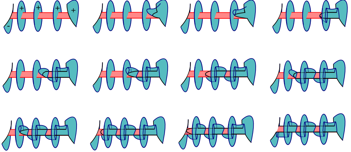
Figure 3.24: Left to right, top to bottom: One leaf in a band movie \mathcal{G}_t as t decreases from 1 to 0.
