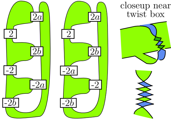
Figure 6.5: Minimum-genus surfaces for knots in Families 2 and 3. These are fibers if and only if |a| = |b| = 1 , so a knot in Family 2 or 3 is fibered if and only if |a| = |b| = 1 .
