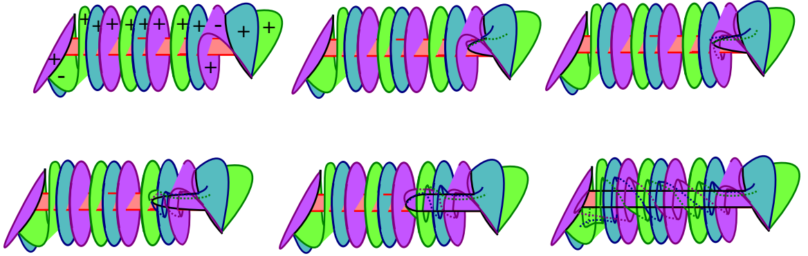
Figure 3.25: Left to right, top to bottom: Three leaves in a band movie \mathcal{G}_t as t decreases from 1 to 0.
