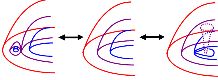
Figure 3.3: As t decreases, we stabilize or destabilize \mathcal{F}_t at a point in \partial h^{-1}(t) .
