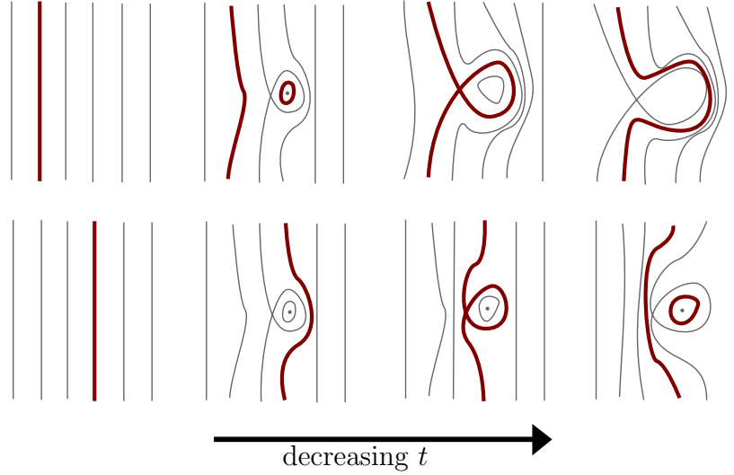
Figure 3.2: Each row is a schematic of an interior stabilization movie (either index-0,-1 or -2,-3). In the top movie, the cone is type I and the dot is type \emptyset . In the bottom, the cone is type II and the dot is type III.
