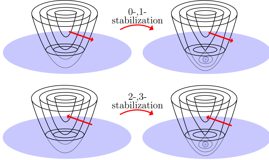
Figure 3.28: Leaves near a dot in the singularity \mathcal{G}_t induces on D . The red arrow indicates the positive S^1 direction of \mathcal{G}_t . We stabilize, and choose the indices of the stabilization as indicated.
