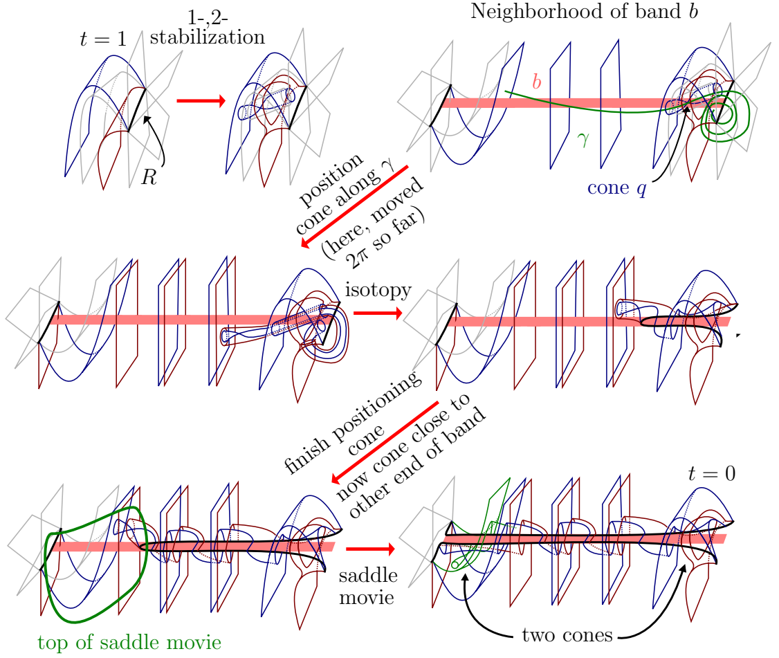
Figure 3.23: Some leaves of \mathcal{G}_t (a band movie) near a neighborhood of band b . Outside this neighborhood, \mathcal{G}_t = \mathcal{G}_1 for all t .
