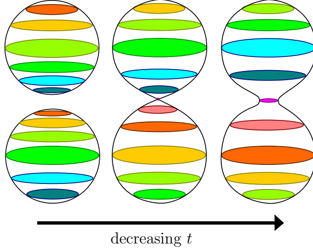
Figure 3.9: The fourth boundary fusion movie.
