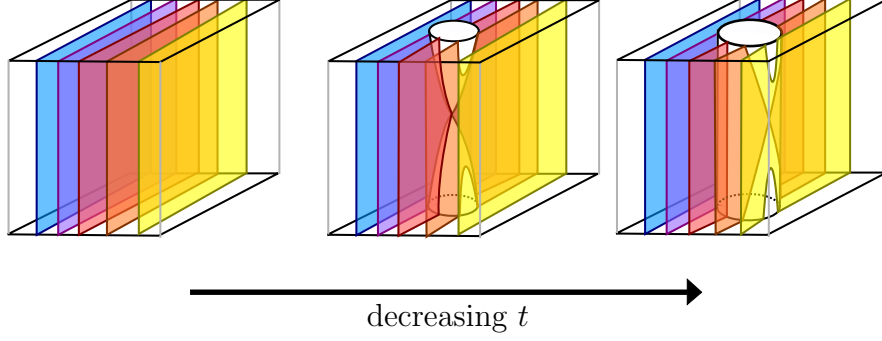
Figure 3.6: The first boundary fusion movie.
