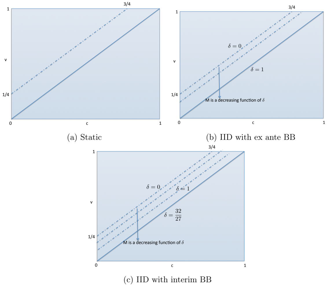
Figure 2.1: No-trade regions
