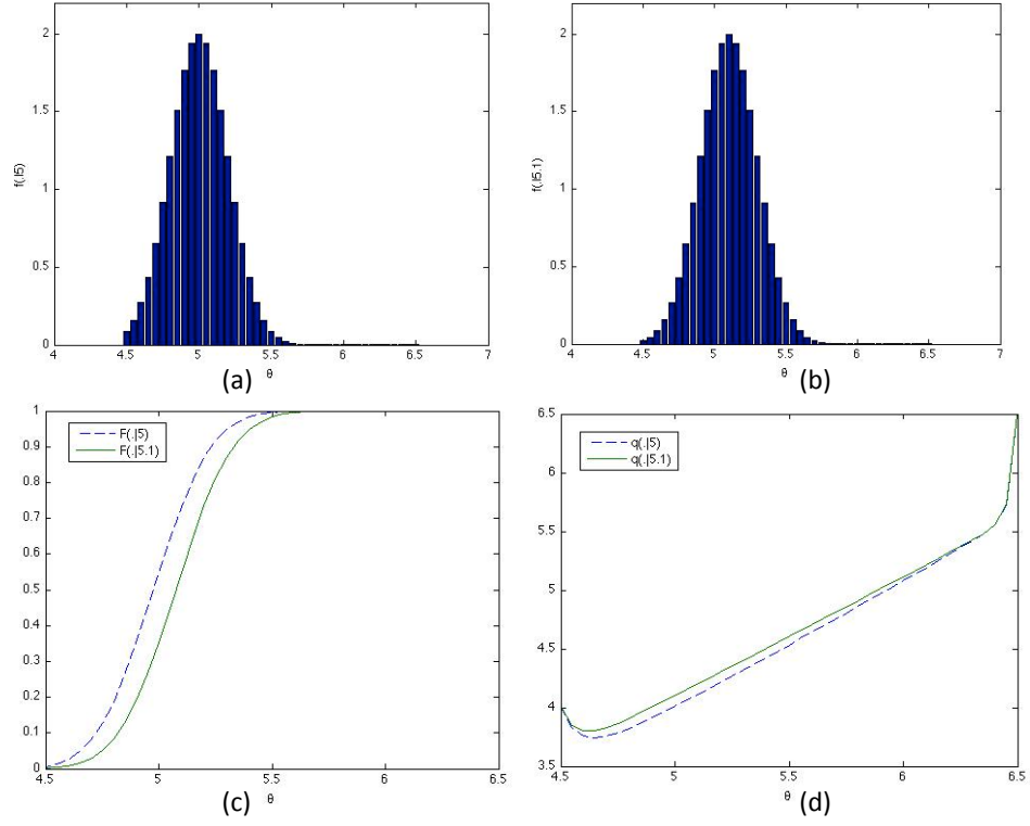
Figure 3.3: Example 8, the exponential case. \alpha = 2 , \Delta\theta = 0.05 .
