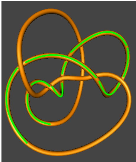
Figure 5.12: The knot obtained by resolving two crossings in K_n .
