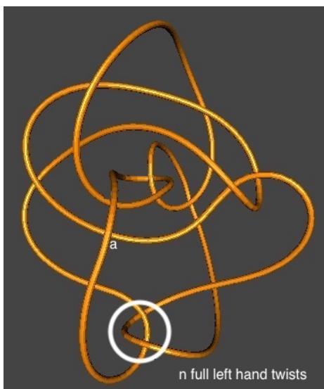
Figure 5.1: Knot K_1 as shown. The knot K_n has n full left hand twists inside the white circle.
