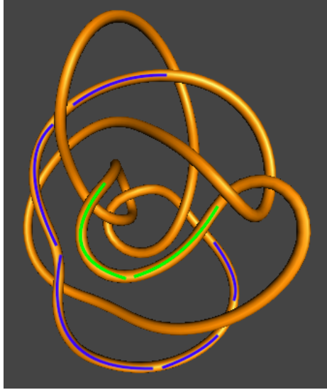
Figure 5.11: The knot obtained by resolving two crossings in K_n .
