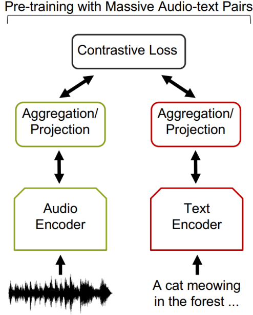
Figure 4.1: The baseline bi-encoder model architecture (from [36]).
