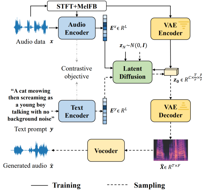
Figure 4.2: The AudioLDM architecture for Text-to-Audio Generation (from [24]).
