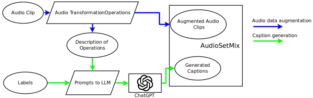
Figure 3.1: The overall pipeline to generate the AudioSetMix.
